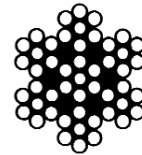
(7 x 7)
